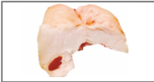
Fat tail
